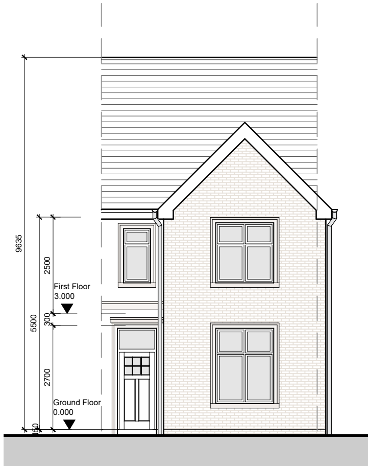
Front Elevation
