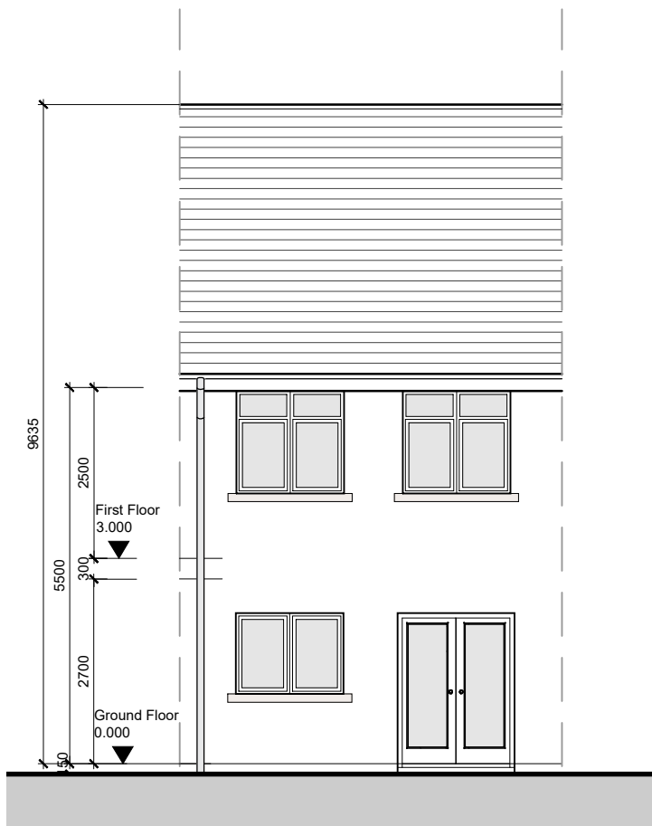
Rear Elevation
